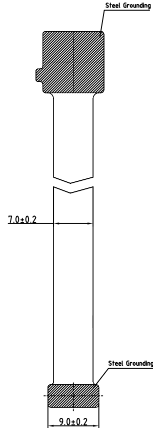
BOTTEM VIEW
